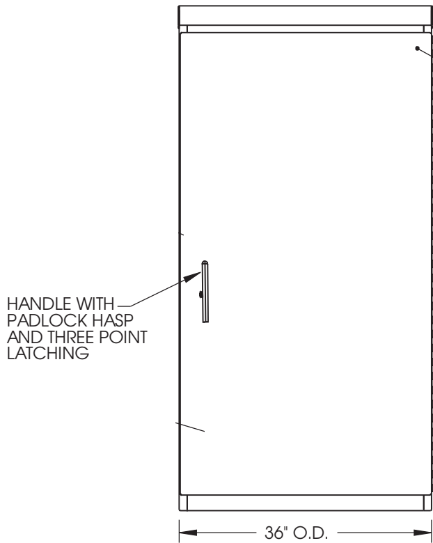
FRONT VIEW
